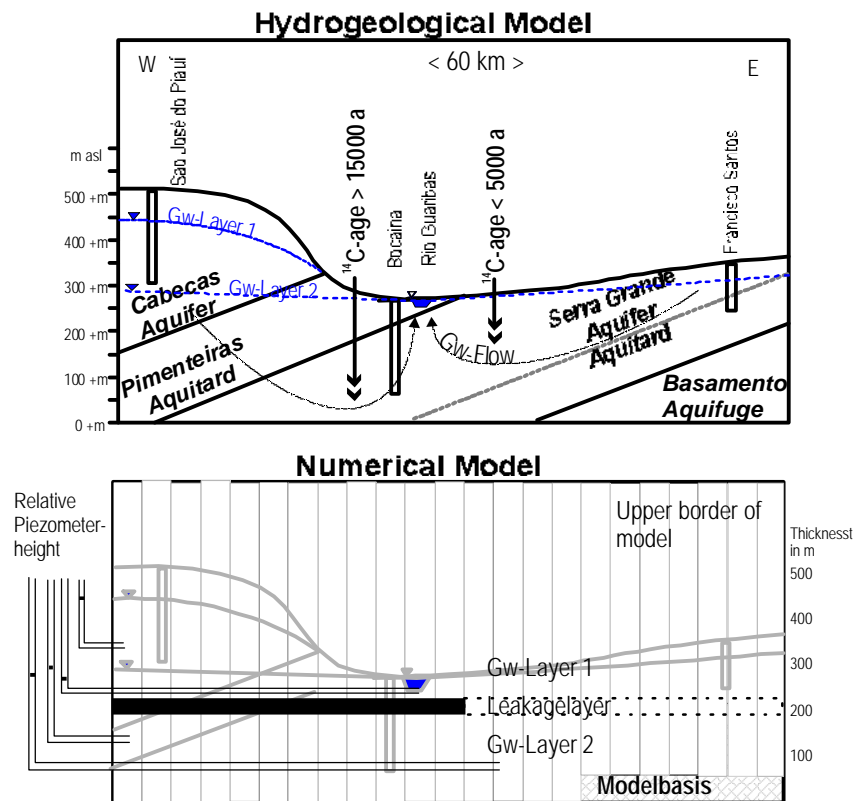
Figure 2: Hydrogeological model with 14 C-dated groundwaters and the translation into a numerical groundwater model with MODFLOW
