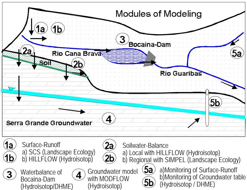
Figure 1: Structure and involved working groups of the water balance method WARIG
