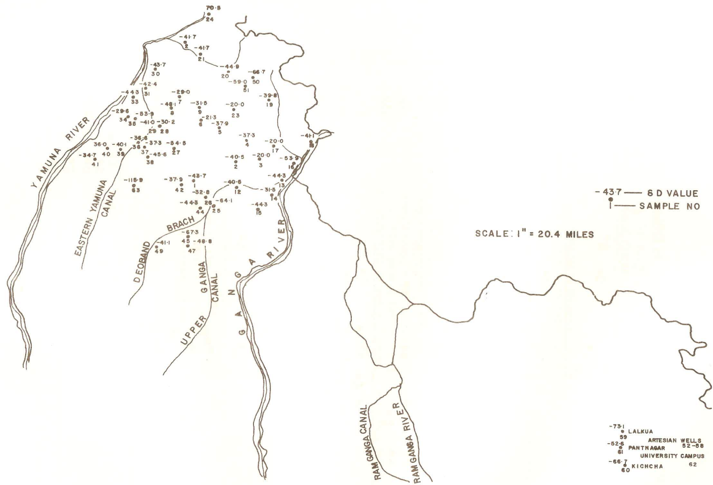
FIGURE 3 - Deuterium contents of ground waters in northern Uttar Pradesh, India
