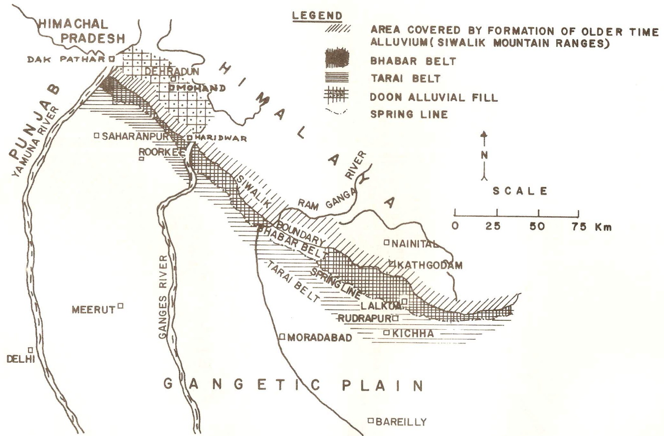
FIGURE 1 - Geological classification of the deuterium-inventory area
