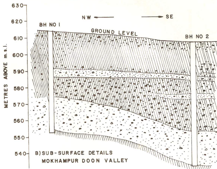
FIGURE 2 - Typical sub-surface details in "Tarai-Bhabar" and Doon Valley
